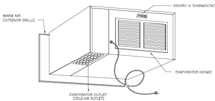
EWKCE air intake and exhaust diagram
